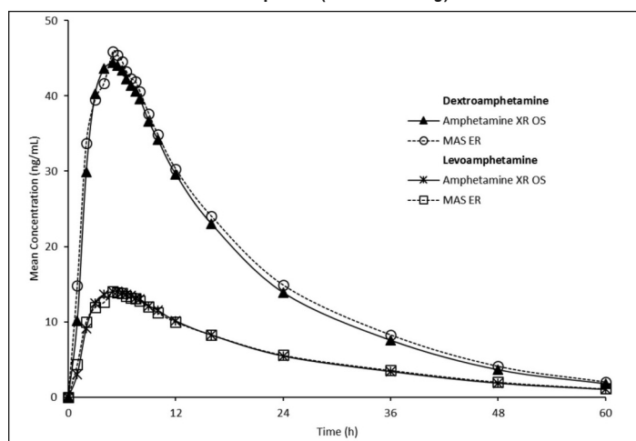
Figure 1: Mean Concentration of D-Amphetamine and L-Amphetamine vs Time for a 15 mL Dose of ADZENYS ER (18.8 mg amphetamine base equivalent) and Mixed Salts of a Single-Entity Amphetamine Product Extended-Release Capsules (MAS ER 30 mg) in the Fasted State
